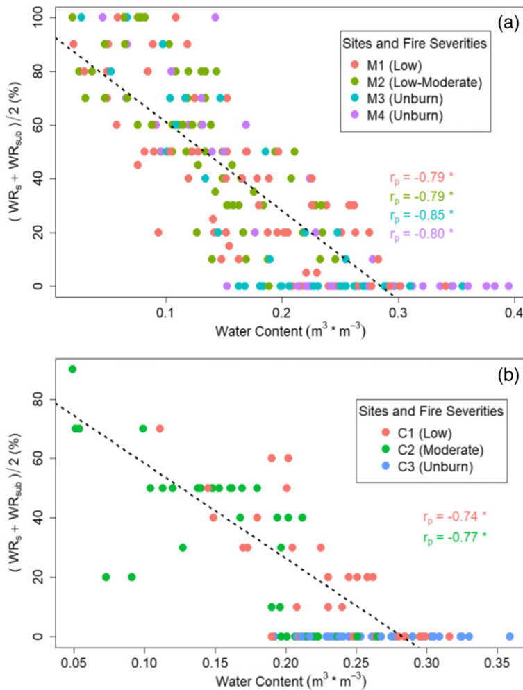
FIGURE 6 Relationship between soil water repellency (average of surface and subsurface, that is, (WR_s + WR_{sub})/2 ) and water content in (a) Mount Pleasant and (b) Chimney Rock. r_p refers to the Pearson's correlation coefficient for each site, whereas an asterisk (*) indicates a significant correlation between soil water and water content ( p < .05 ). Dashed line shows the significant overall linear regression using analysis of covariance; individual linear regression models were not significantly different between sites ( p_{slope} = 0.22 and p_{intercept} = 0.42 in Mount Pleasant; p_{slope} = 0.17 and p_{intercept} = 0.07 in Chimney Rock)
