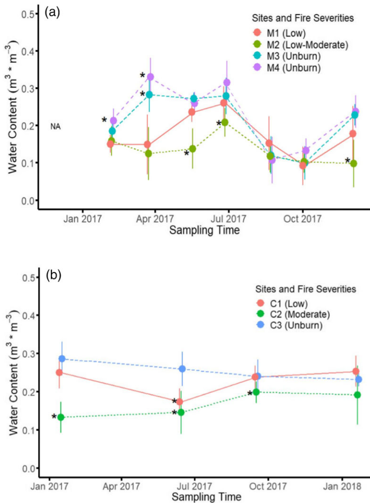
FIGURE 4 The variations of soil water content in each sampling time after wildfires in Mount Pleasant (a) and Chimney Rock (b). “NA” indicates times when measurements were not recorded. Bars show standard deviations, whereas an asterisk (*) indicates significant differences from other sites within the same sampling time (ANOVA with Tukey's HSD, p < .05 ). ANOVA, analysis of variance; HSD, honestly significant difference
