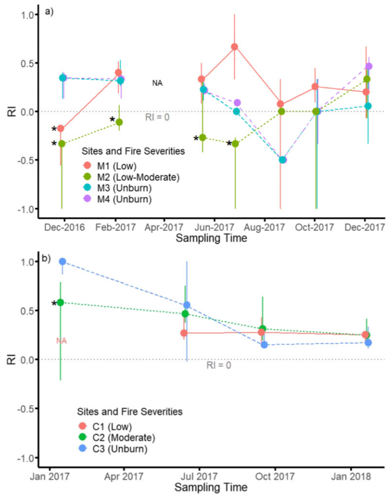
FIGURE 5 Relative infiltration rates ( RI ) for each sampling time after wildfires in (a) Mount Pleasant and (b) Chimney Rock. “NA” indicates times and sites where measurements were not collected. Points refer to the median and bars indicate 95% confidence intervals, whereas an asterisk (*) indicates significant difference from other sites within the same sampling time (K-W with MU, p < .05 ). K-W, Kruskal–Wallis test; MU, Mann–Whitney U test
