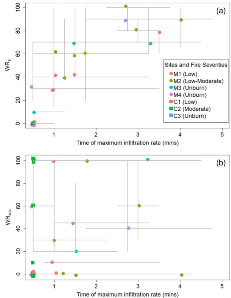
FIGURE 7 The relationship between the time of maximum infiltration rate ( t_{mir} ) and water repellency in the (a) surface and (b) subsurface layers. Data come from both sampling locations: Mount Pleasant (M) and Chimney Rock (C). Dots/squares refer to the median, and bars indicate 95% confidence intervals
