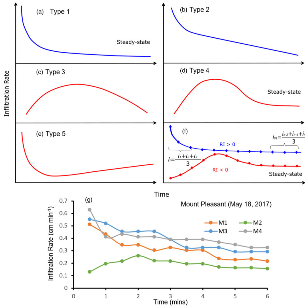
FIGURE 1 Conceptual infiltration curves for hydrophilic and water-repellent soils, based on previous research by Imeson et al. (1992) and Pierson, Robichaud, and Spaeth (2001): (a) Type 1: exponential decrease; (b) Type 2: linear decrease; (c) Type 3: initial increase to decrease; (d) Type 4: initial increase to steady state; and (e) Type 5: exponential decrease to linear increase. Panel (f) presents the calculation for relative infiltration (RI) based on initial ( i_i ) and steady-state ( i_{ss} ) infiltration rates, whereas Panel (g) shows example hydrographs that were collected in the Mount Pleasant location on May 18, 2017. Note that the blue lines in panels a–f represent infiltration curves associated with hydrophilic soil conditions, whereas the red lines indicate water-repellent soil conditions
