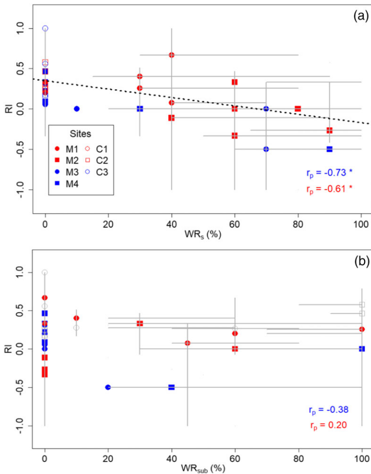
FIGURE 8 Relationship between relative infiltration rates ( RI ) and water repellency in (a) surface ( WR_s ) and (b) subsurface layers ( WR_{sub} ) in Mount Pleasant (M) and Chimney Rock (C). Dots/squares refer to the median, and bars indicate 95% confidence intervals. r_p refers to the coefficient of determination using Pearson's correlation coefficient in burned and unburned sites, whereas an asterisk (*) indicates a significant correlation between RI and either WR_s or WR_{sub} ( p < .05 ). Dashed line shows significant overall linear regression using analysis of covariance; individual linear regression models were not significantly different between burned and unburned sites ( p_{slope} = 0.20 and p_{intercept} = 0.14 )
